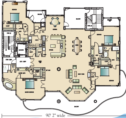
TYPICAL EAST & WEST TOWERS FLOOR PLANS
